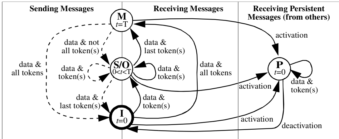
(a) Processor
