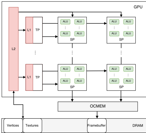
Fig. 2: Building blocks of an integrated GPU
