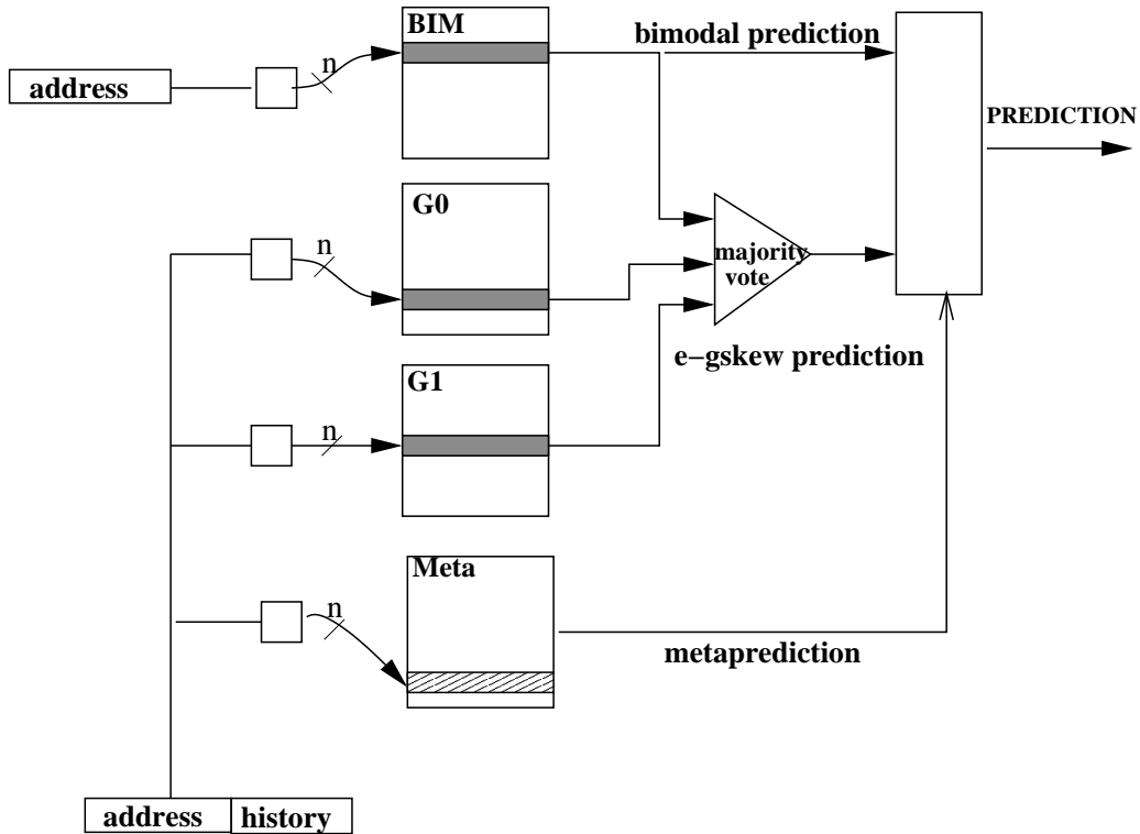
Figure 1. The 2bcgskew branch predictor
