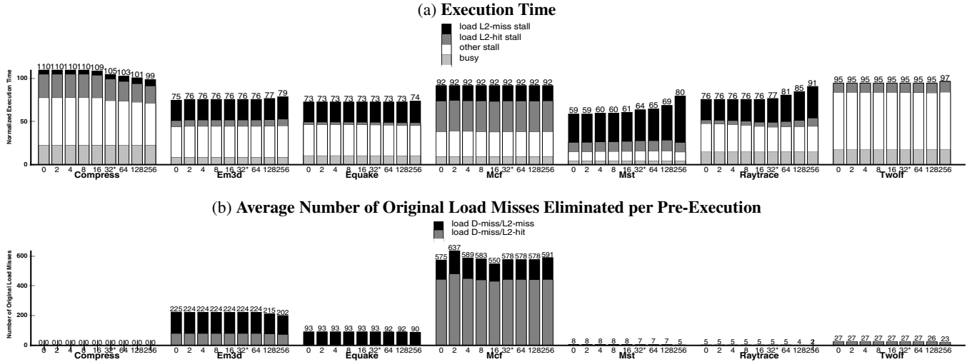
Figure 8. Performance of pre-execution with various thread-spawn latencies ( X = X cycles; our baseline is 32^* ). Part (a) shows the execution time. Part (b) shows the average number of original load misses eliminated per pre-execution.
