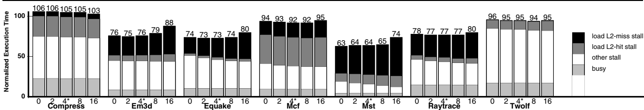
Figure 7. Performance of pre-execution with different thread prioritization ( X = adding X to the “ICOUNT” of each pre-execution thread; our baseline is 4*). Note that higher ICOUNT values mean lower priorities. Execution time is normalized to the original case.
