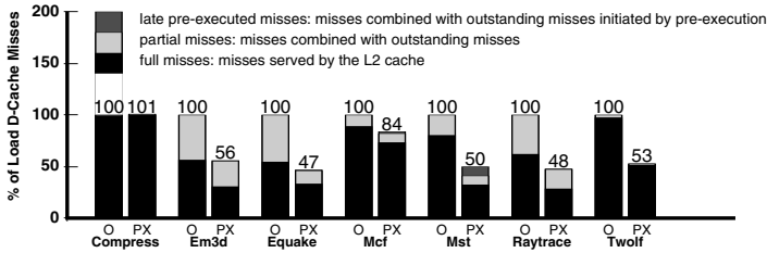
Figure 5. Performance of software-controlled pre-execution (O = original, PX = pre-executed)
