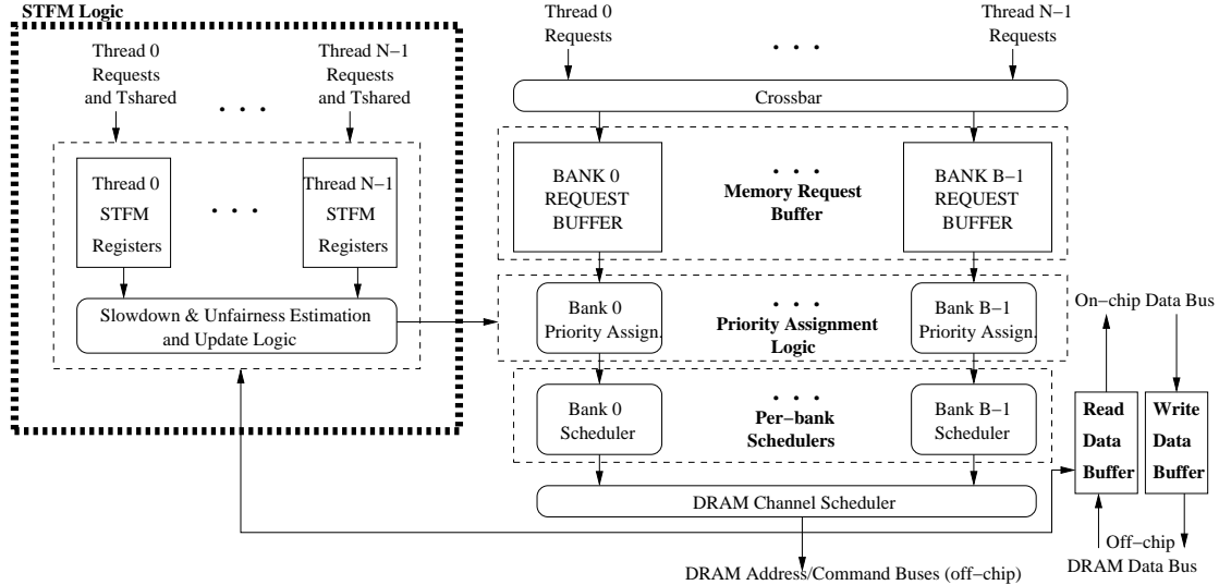
Figure 4. Organization of the on-chip STFMs memory controller. Only major control and data paths are shown to keep the figure simple.
