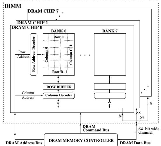
Figure 2. High-level organization of a DRAM system
