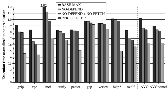
Figure 2. Execution time when sources of overhead in predicated execution are ideally eliminated.
