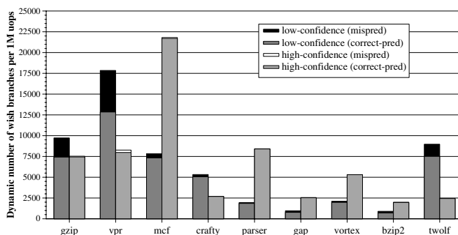
Figure 11. Dynamic number of wish branches per 1M retired \mu ops. Left bars: low-confidence, right bars: high-confidence.
