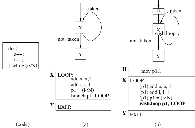
Figure 4. do-while loop source code and the corresponding control flow graphs and assembly code for (a) normal backward branch code (b) wish loop code.
