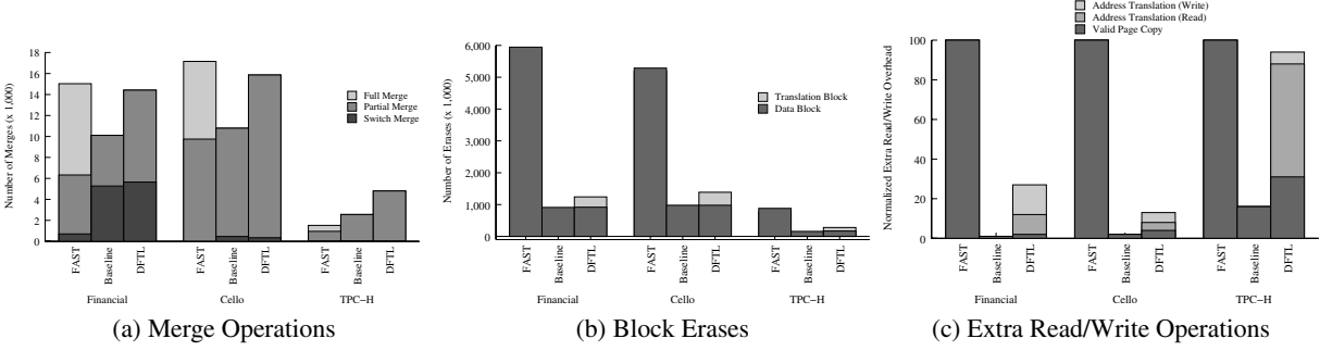
Figure 6: Overheads with different FTL schemes. We compare DFTL with FAST and Baseline for three workloads: Financial, Cello99, and TPC-H. The overheads for the highly read-oriented Web Search workload are significantly smaller than others and we do not show them here. In (c), Address Translation (Read) and Address Translation (Write) denote the extra read and write operations for address translations required in DFTL, respectively. All extra read/write operations have been normalized with respect to FAST FTL scheme.
