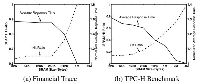
Figure 11: Impact of SRAM size on DFTL. Response times have been normalized with respect to the Baseline FTL scheme. For both the Financial trace and TPC-H, there is performance improvement with increased SRAM hit-ratio. However, beyond the working-set size of workloads there is no benefit of additional SRAM for address translation. The 99% confidence intervals are very small and hence not shown.
