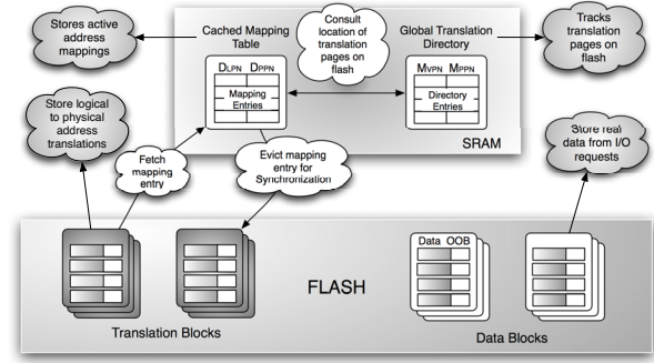
Figure 4: Schematic Design of DFTL. D_{LPN} : Logical Data Page Number, D_{PPN} : Physical Data Page Number, M_{VPN} : Virtual Translation Page Number, M_{PPN} : Physical Translation Page Number.
