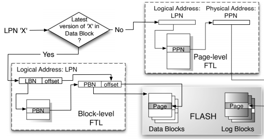
Figure 1: Hybrid FTL Scheme, combining a block-based FTL for data blocks with a page-based FTL for log blocks. LPN: Logical Page Number, PPN: Physical Page Number, LBN: Logical Block Number, PBN: Physical Block Number.
