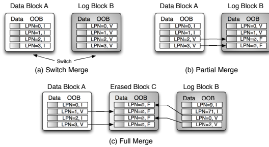
Figure 2: Various Merge operations (Switch, Partial, and Full) in log-buffer based FTL schemes. V: Valid, I: Invalid, and F: Free/Erased and LPN is Logical Page Number.
