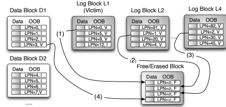
Figure 3: Expensive Full Merge.
