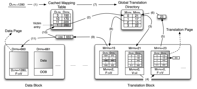
Figure 5: (1) Request to D_{LPN} 1280 incurs a miss in Cached Mapping Table (CMT), (2) Victim entry D_{LPN} 1 is selected, its corresponding translation page M_{PPN} 21 is located using Global Translation Directory (GTD), (3)-(4) M_{PPN} 21 is read, updated ( D_{PPN} 130 \rightarrow D_{PPN} 260) and written to a free translation page ( M_{PPN} 23), (5)-(6) GTD is updated ( M_{PPN} 21 \rightarrow M_{PPN} 23) and D_{LPN} 1 entry is erased from CMT. (7)-(11) The original request's ( D_{LPN} 1280) translation page is located on flash ( M_{PPN} 15). The mapping entry is loaded into CMT and the request is serviced. Note that each GTD entry maps 512 logically consecutive mappings.
